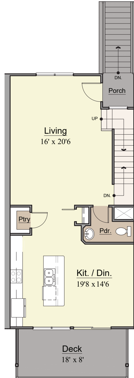
Main Floor Plan
